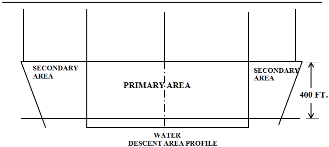
Figure 5.6.1.3. REDA Dimensions (Profile View)
