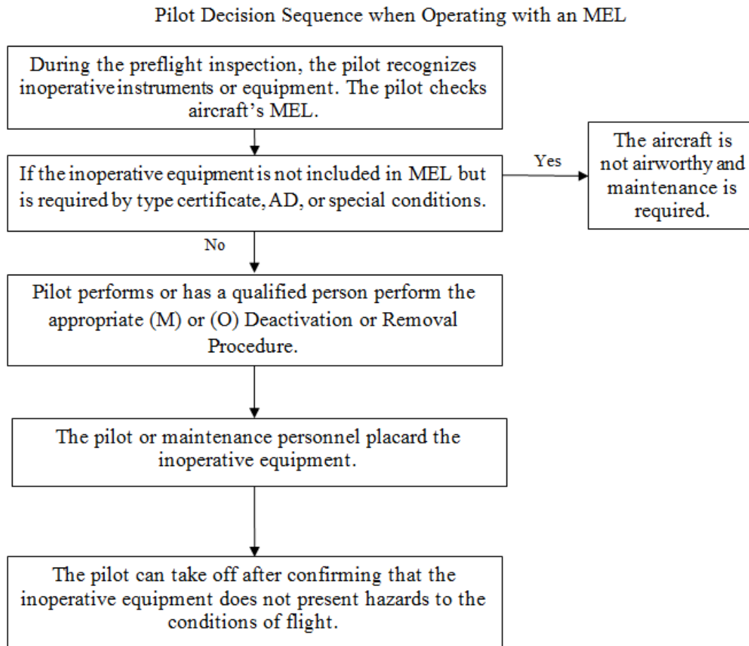
Figure 5.4.1.4. Flowchart - Operating With an MEL
